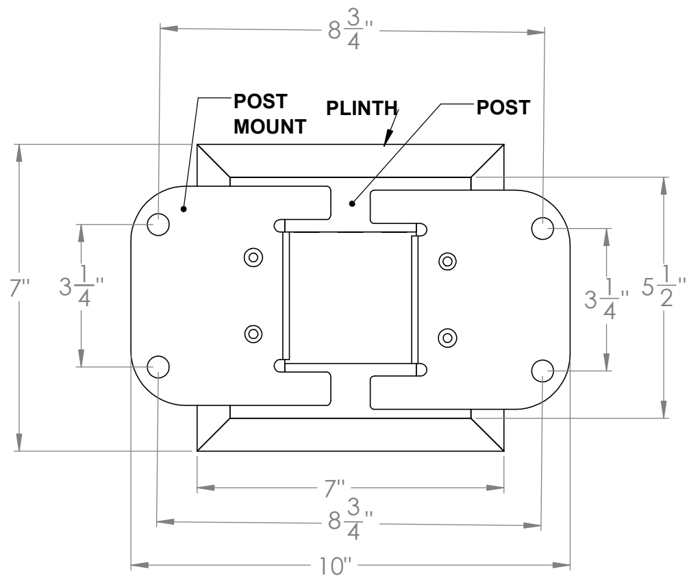
POST DETAIL
